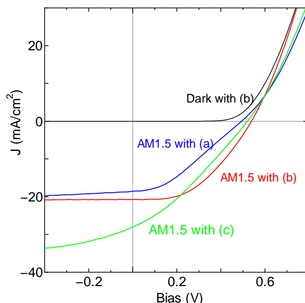
Fig. 3 Solar cell J-V characteristics of cells by SWNTs morphologies (a), (b) and (c) in Fig. 1 under AM1.5 illumination and morphology (b) in dark.
