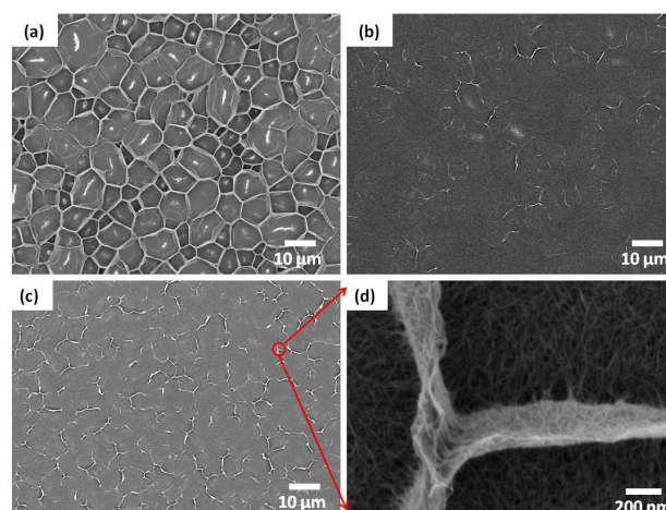
Fig. 1 (a, b, c) SEM images of different self-organizing micro-honeycomb network of SWNTs; (d) enlarged image of condensed SWNTs bundles from (c).
