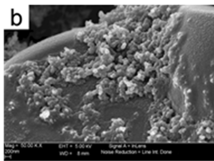
Figure 1. SEM images of the cathodes containing coated LiCoO 2 particles.
